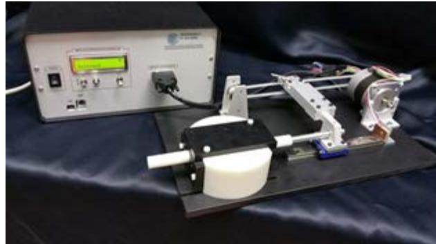
Figure 2: Photo of the switchable phantom kit.
